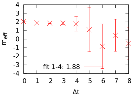
U_1: \phi^{(1)*}\phi^{(1)}
