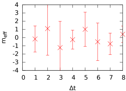
F_1: \phi^{(1)}
